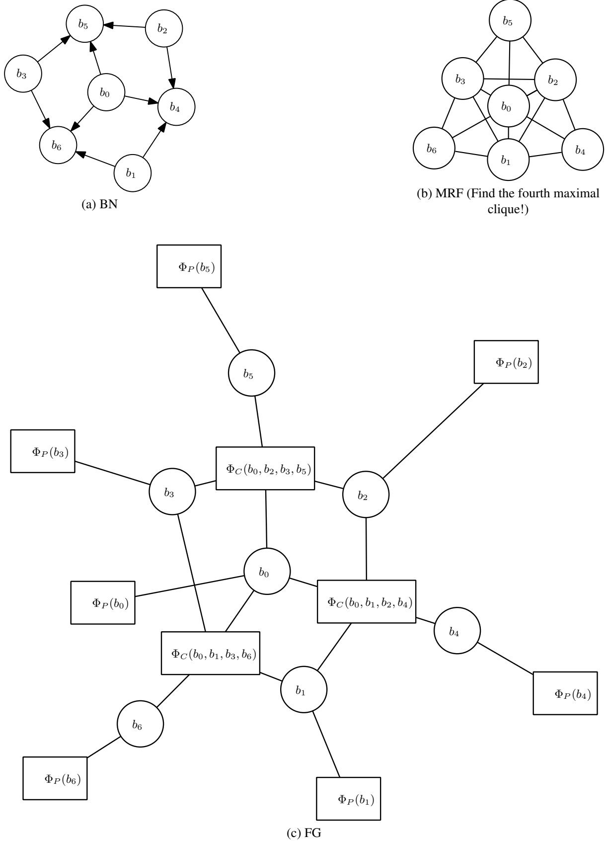
Figure 2: Various PGM representations for the Hamming (7,4) coding stage.
